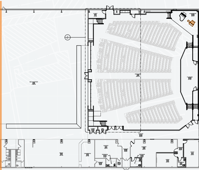
2 MEZZANINE LEVEL 77' 0" x 111' 0"
